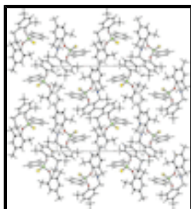
Fig. 2. Packing view of the molecules in the unit cell.
